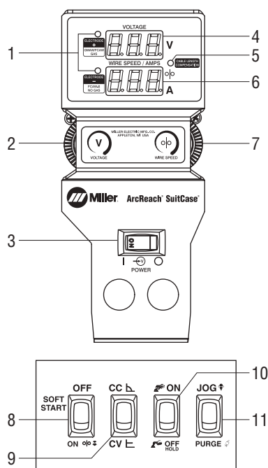
Panel de control interno
